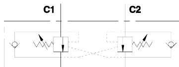
Dobbelt Overcenter vent
