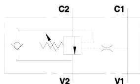
Overcenter vent
